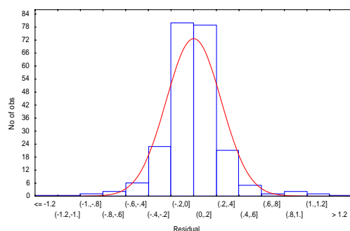
Fig. 3 Histogram of model residuals
