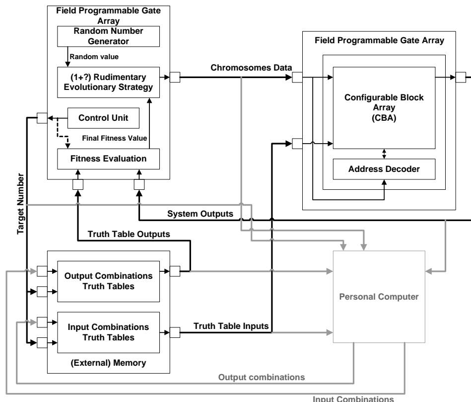
Fig. 8 Multi-board functional-level RTC top-level architecture
