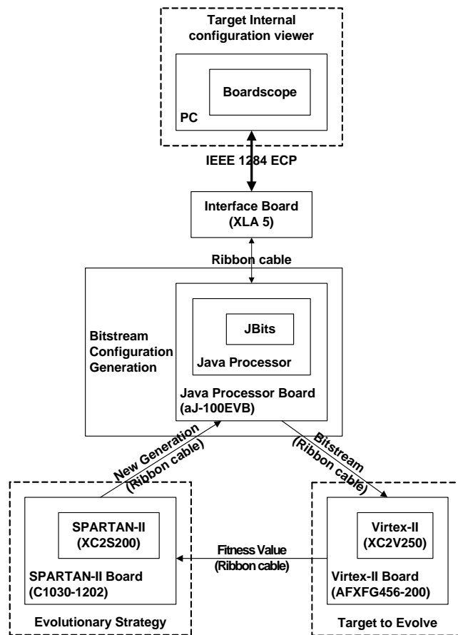
Fig. 7 JBits RTC top-level architecture
