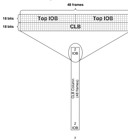
Fig. 4 CLB column detailed [22]
