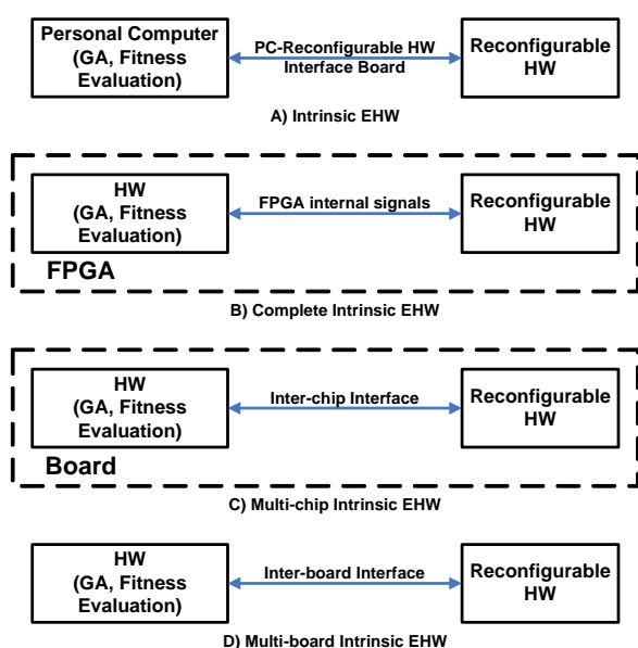
Fig. 1 Type of Implementation of Intrinsic EHW system
