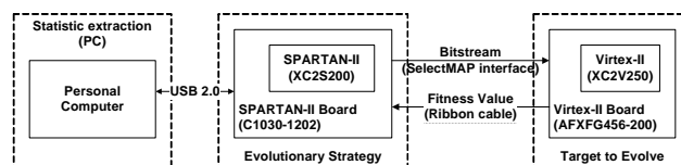
Fig. 6 FPGA-based Run-Time Configuration system architecture
