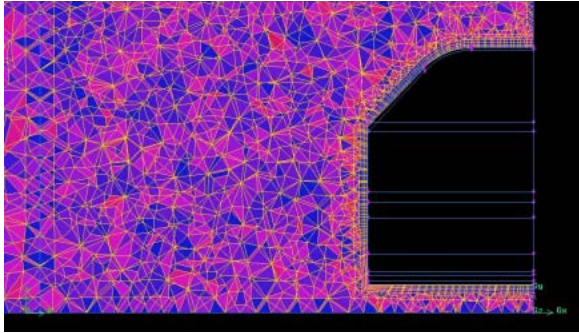
Fig. 2 Layer of prism element in Gambit
