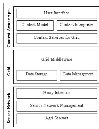
Fig. 2 Context-Aware Sensor Grid Framework for Agriculture
