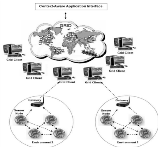
Fig. 1 Context-Aware Sensor Grid Architecture
