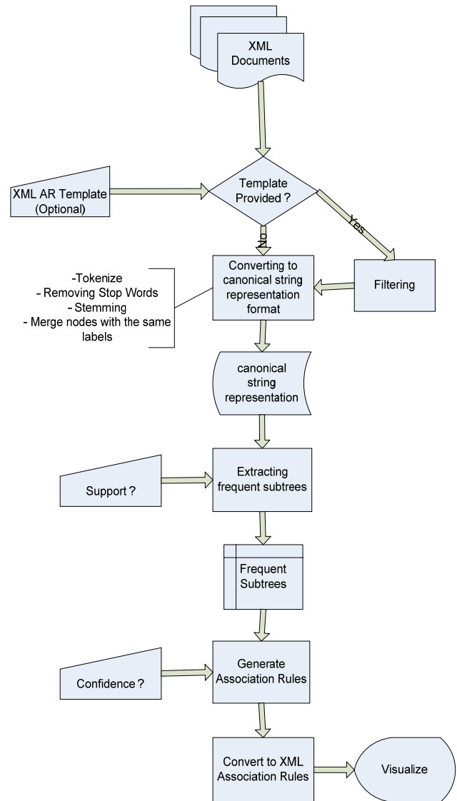
Fig. 3 Association Rule Mining from XML documents
