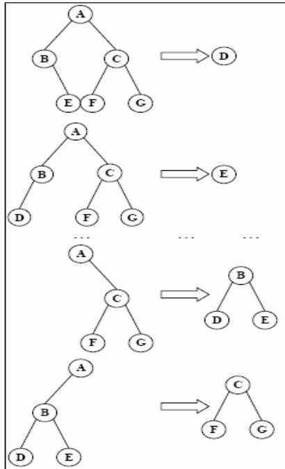
Fig. 4 Generating Association Rules from Frequent Subtrees
