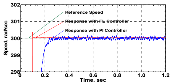
Fig. 5 Enlarged speed response comparison at no-load
