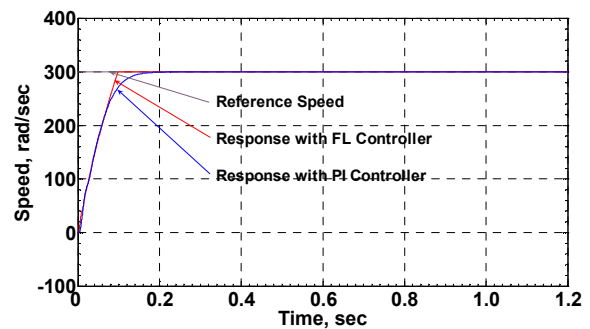
Fig. 4 Speed response comparison at no-load
