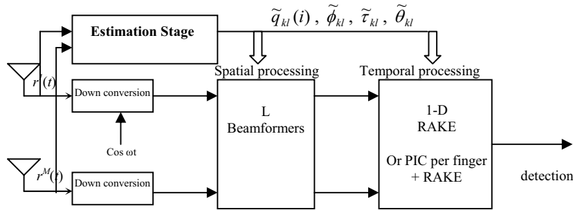
Fig. 2. 2D-RAKE receiver
