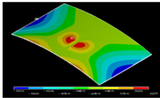
Fig. 5: Difference between global buckling of cases 1 and 2
