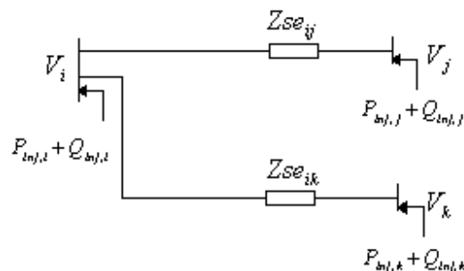
Fig. 3 Power injection model of two converter IPFC
