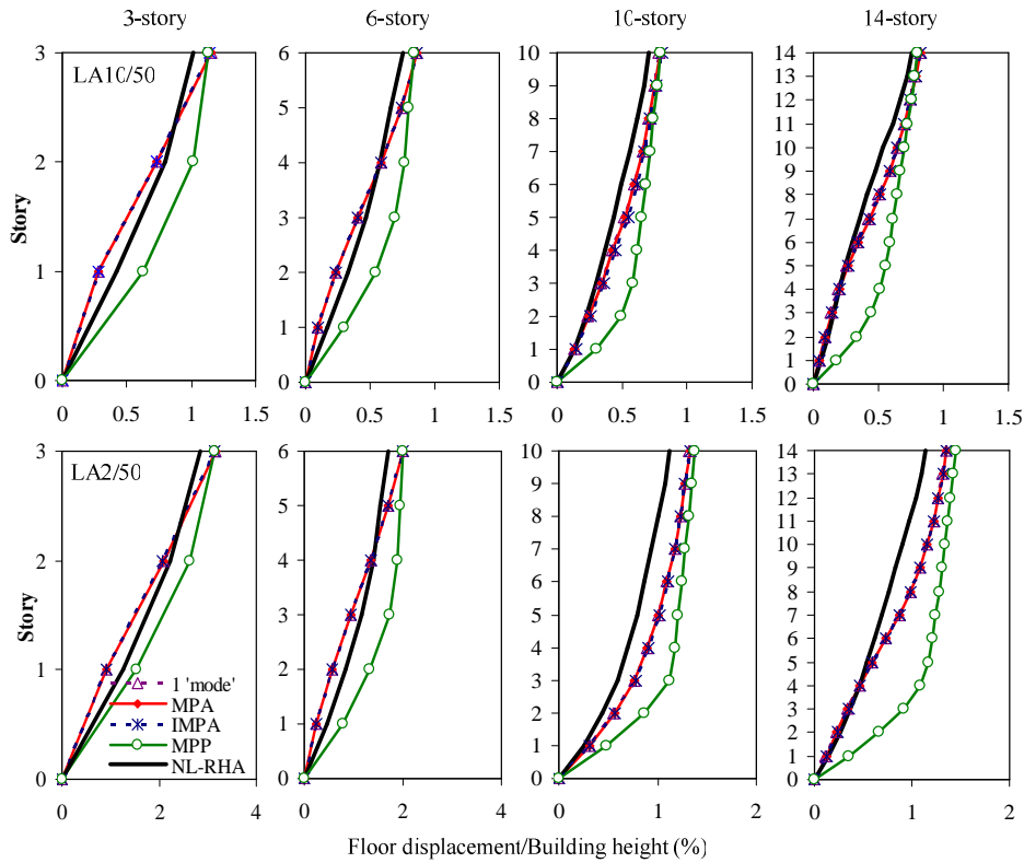
Fig. 5 Median floor displacements of 3-, 6-, 10- and 14-story buildings determined by one 'mode' pushover analysis, MPA, IMPA, MPP and NL-RHA due to LA10/50 (first row), and LA2/50 (second row) ground motions
