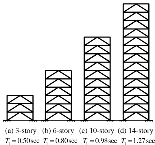
Fig. 1 Frame elevations of 3-, 6-, 10-, and 14-story buildings
