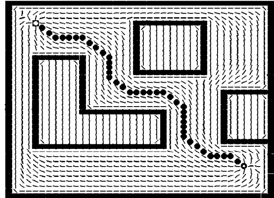
(b) Path generated with Neumann boundary condition after 500 iterations
