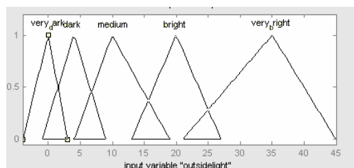
Fig. 2 Membership function of outside light
