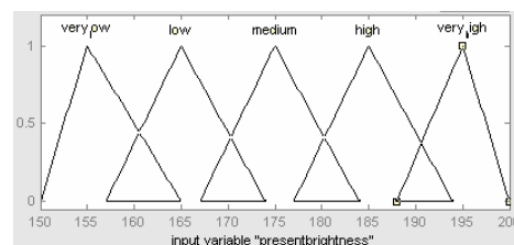
Fig. 3 Membership function of grid voltages
