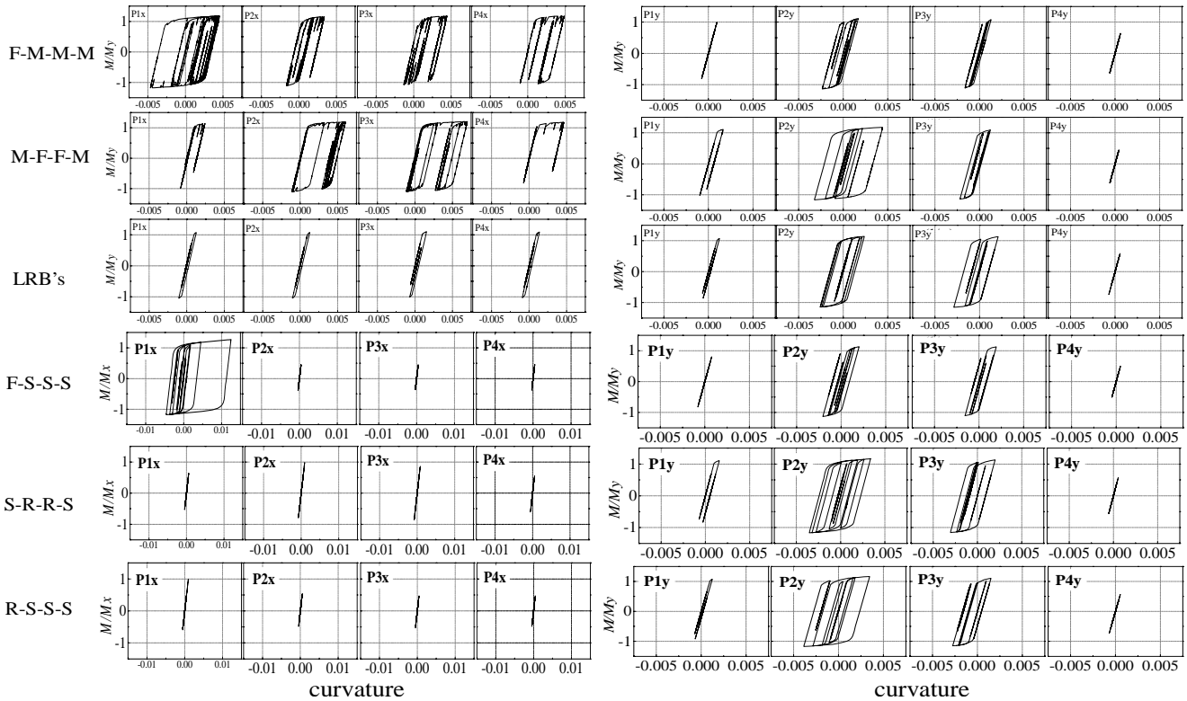
Fig. 6 Curvature moments at pier's bottom
