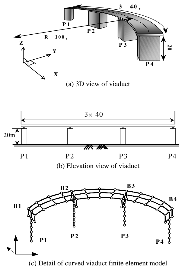
Fig. 1 Model of curved highway viaduct
