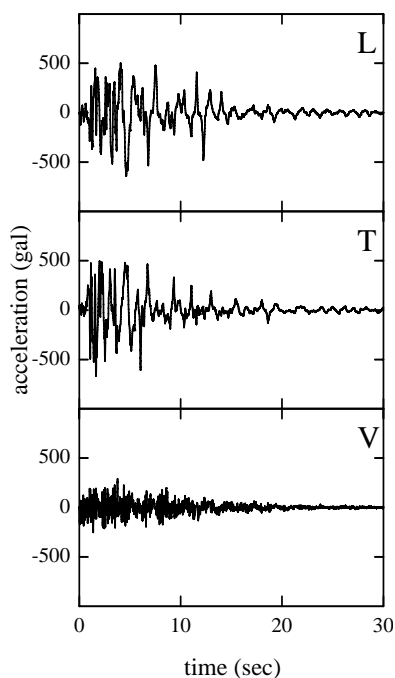
Fig. 4 JR Takatori St. Record, 1995 Kobe Earthquake.
