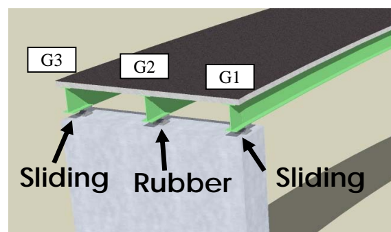
Fig. 2 Hedge reaction force bearing system(R)
