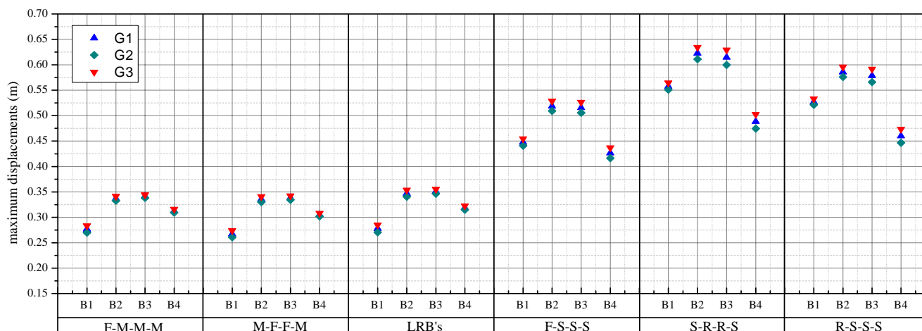
Fig. 5 Maximum deck displacements on superstructure
