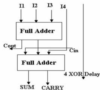
Fig. 1 Four to two counter using full adders
