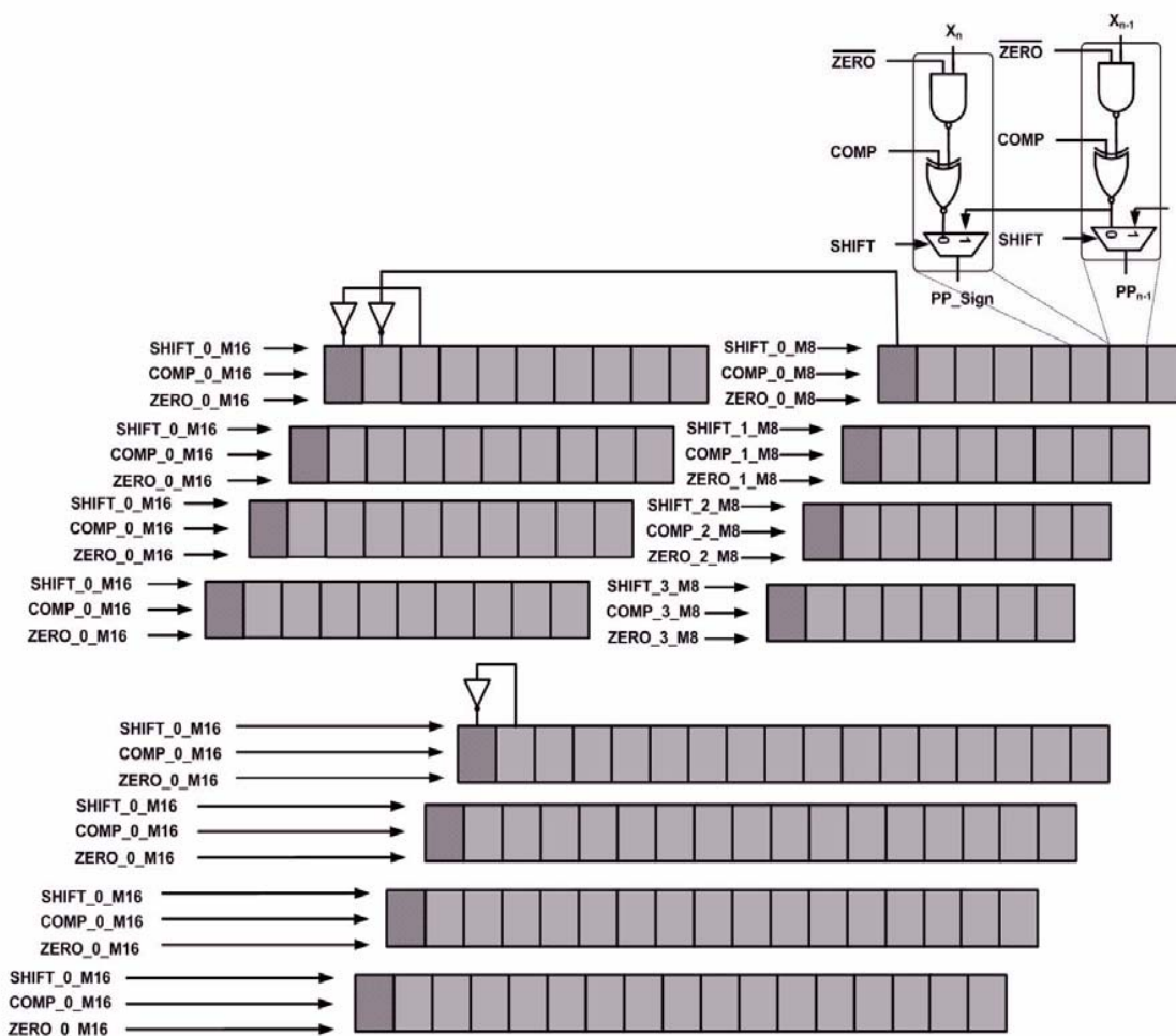
Fig. 4 Inner product generator
