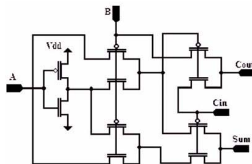
Fig. 2 A novel full adder
