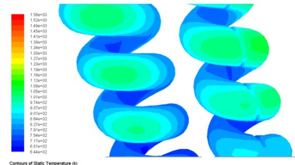
Fig. 14 Contours of static temperature for cooling ducts having turbulators of e/D = 0.06 and 0.75mm rib thickness
