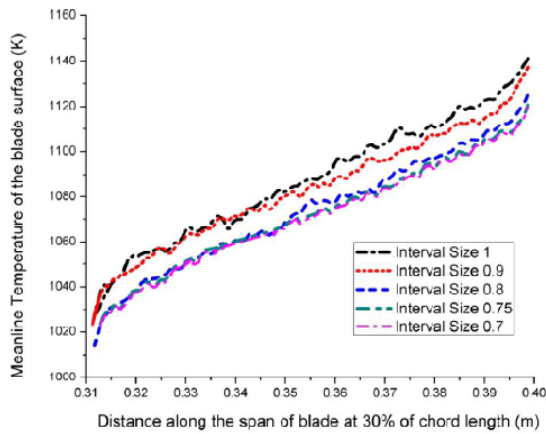
Fig. 3 Results of grid independence test
