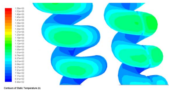
Fig. 20 Contours of Static Temperature for cooling ducts having turbulators of e/D = 0.08 and 0.5mm rib thickness
