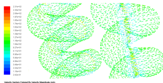
Fig. 24 Velocity vectors for cooling ducts having turbulators of e/D = 0.08 and 0.5mm rib thickness
