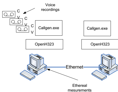
Fig. 2 The facility designed for VoIP streams measurements
