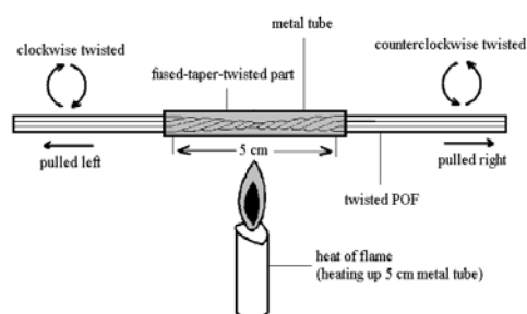
Figure 5. Fabrication method of POFs
