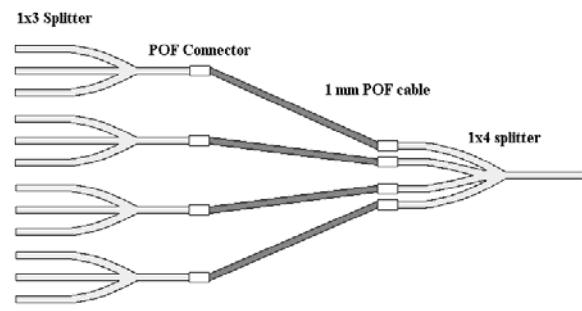
Figure 4. Optical 1x12 coupler design for passive night vision application
