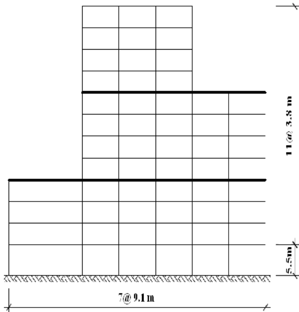
Fig. 6 The 12 storey steel frame
