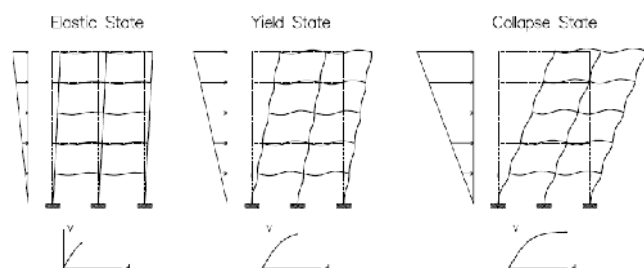
Fig. 1 Yielding sequence through conventional pushover analysis.
