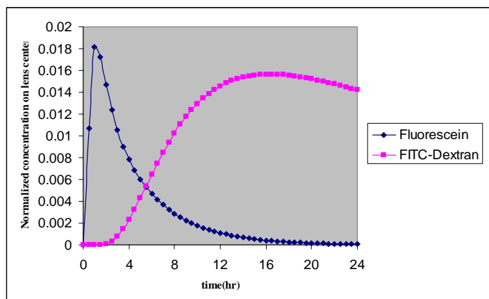
Fig.16 Drug concentration adjacent to the Lens
