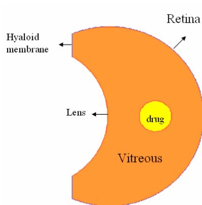
Fig. 2 Geometrical model based on rabbit eye dimension
