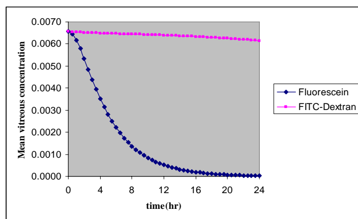
Fig.17 Mean vitreous drug concentration
