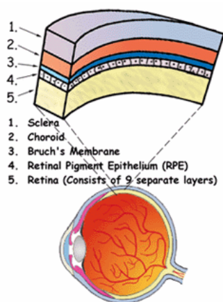
Fig. 5 Schematic view of posterior eye layers
