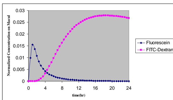
Fig.15 Drug concentration at Macula
