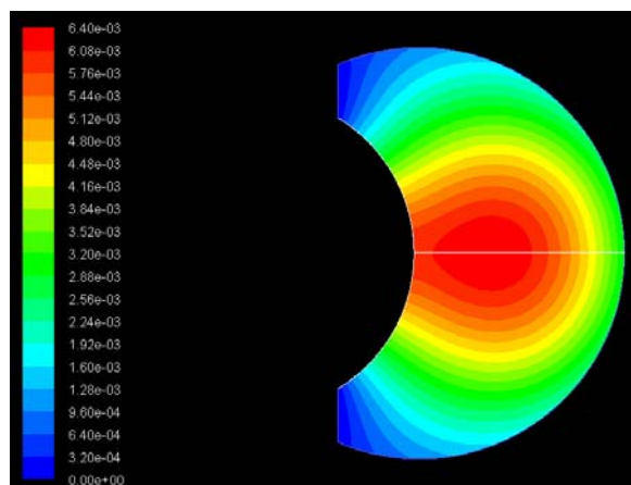
Fig.9 Concentration contour 5hrs after injection of Fluorescein
