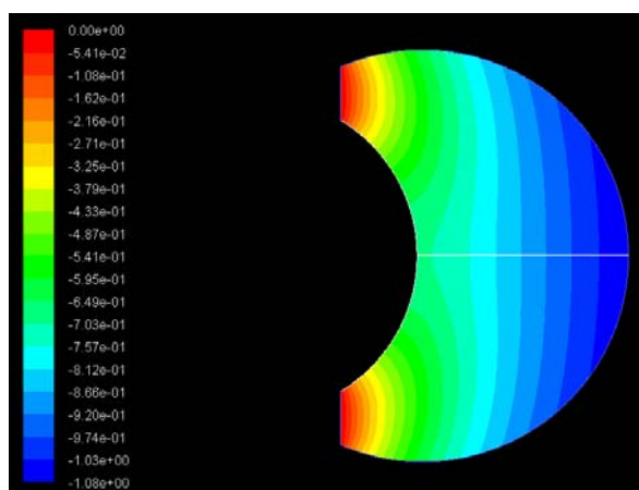
Fig.8 Pressure contour in the vitreous
