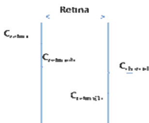
Fig. 6 Schematic of drug concentration on retina layer
