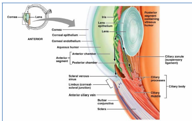
Fig. 4 Secretion of ocular humors from cilliary body
