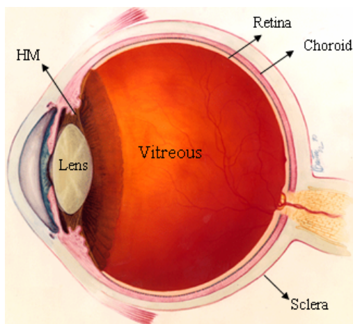
Fig. 1 Anatomy of the human eye
