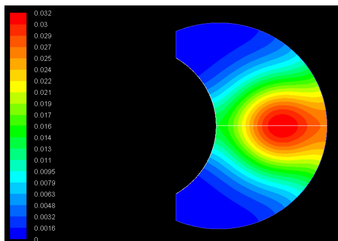
Fig.14 Concentration contour 24hrs after injection of FITC-Dextran
