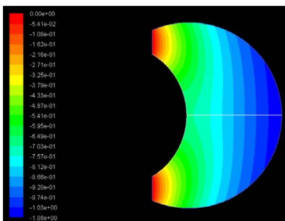
Fig.8 Pressure contour in the vitreous
