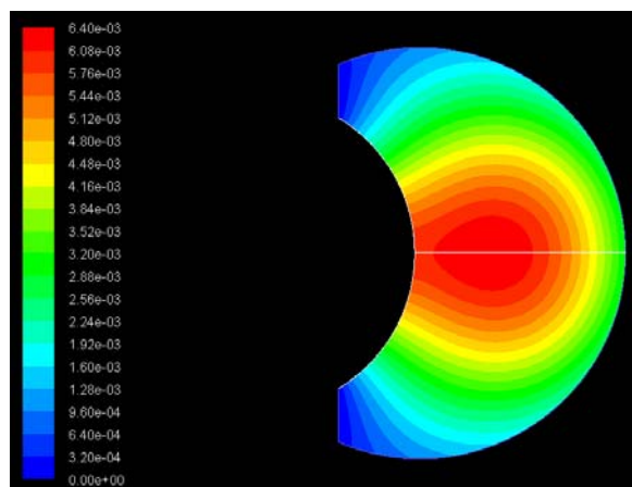
Fig.9 Concentration contour 5hrs after injection of Fluorescein
