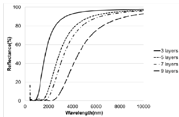
Fig. 1 Simulation spectra of four different metal-dielectric structures
