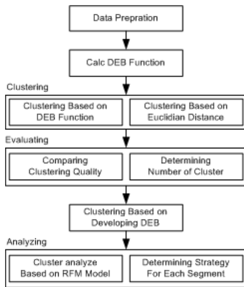
Fig. 1 The proposed Countries Segmentation Methodology
