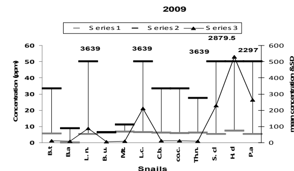
Fig. 9 Tolerance ranges and mean concentration of Lead (Mn) of some fresh water snails collected from River Nile, main branches and canals in Egypt during two years 2008 and 2009, (series1:: min value, series2: max value, series3: mean concentration \pm SD)
