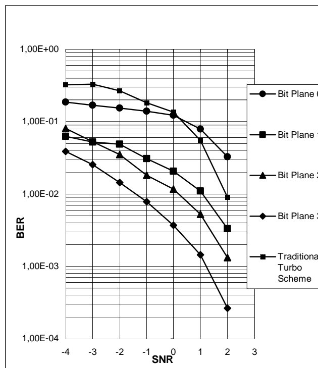
Fig. 7 Bit error performance of conventional Turbo and IC-TS with various bit planes
