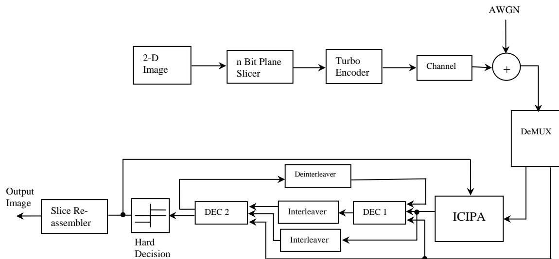
Fig. 1 IC-TS system model
