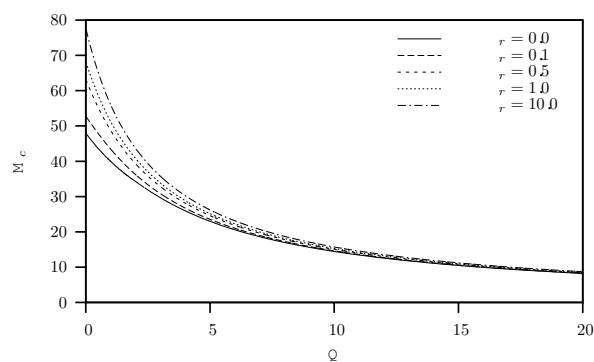
Fig. 8. The critical Marangoni number at the onset of convection as a function of Q , for a range of values of \kappa_r in the case B_i = 0 , and d_r = 1 .
