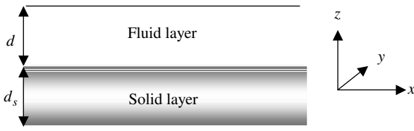
Fig. 1. Geometry of the unperturbed state
