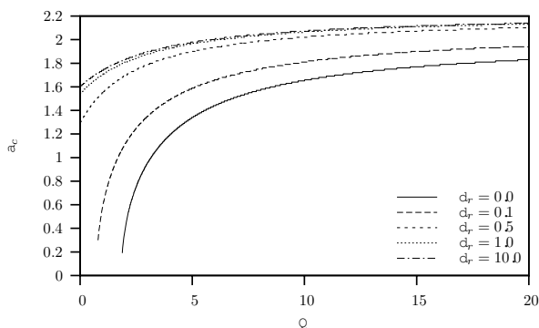
Fig. 7. The critical wave number at the onset of convection as a function of Q , for a range of values of d_r in the case B_i = 0 and \kappa_r = 1 .
