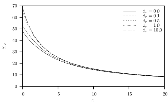
Fig. 6. The critical Marangoni number at the onset of convection as a function of Q , for a range of values of d_r in the case B_i = 0 , and \kappa_r = 1 .
