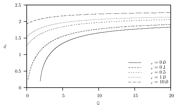
Fig. 9. The critical wave number at the onset of convection as a function of Q , for a range of values of \kappa_r in the case B_i = 0 and d_r = 1 .
