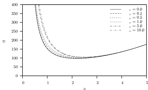
Fig. 5. Numerically-calculated Marangoni number, M as a function of the wave number, a , for various values of \kappa_r , in the case B_i = 2 , d_r = 1 and Q = 1 .
