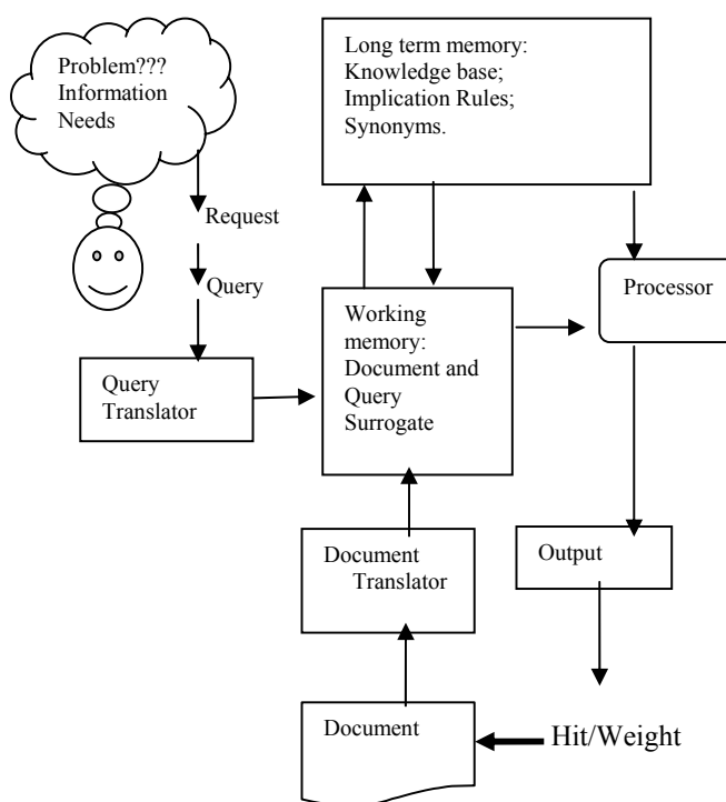
Fig. 1 Information Retrieval System Model
