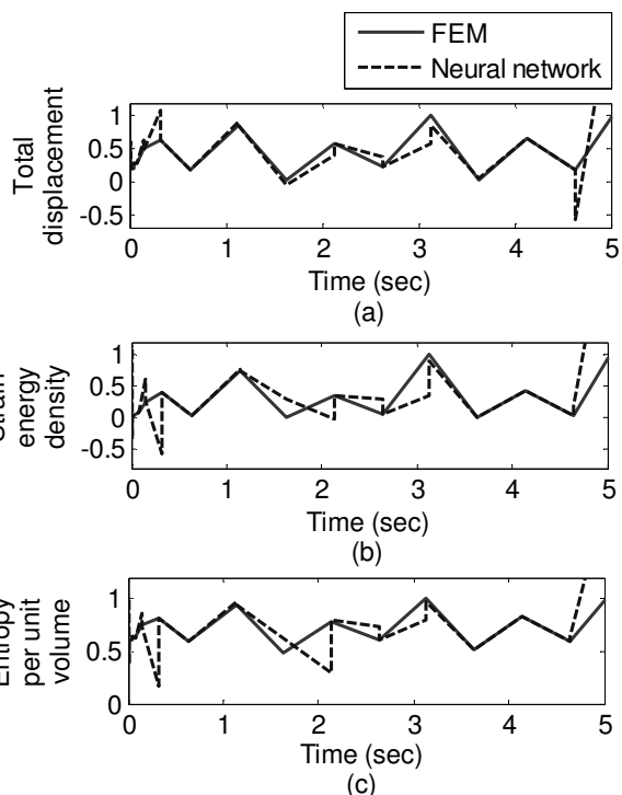
Fig. 5 The variation of normal vessel response such as (a) total displacement, (b) strain energy density and (c) entropy per unit volume shown as a function of time for FEM and ANN model
