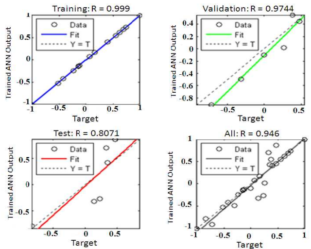
Fig. 9 Training result of proposed network
