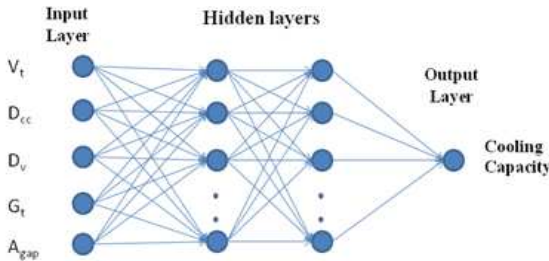
Fig. 8: ANN structure
