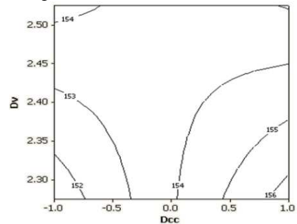
Fig. 6 Contour plot of CC Vs. D_v & D_{cc}
