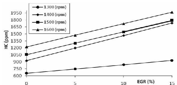
Fig. 5 Effect of EGR on HC emissions of dual fuel HCCI-DI engine at different engine speeds
