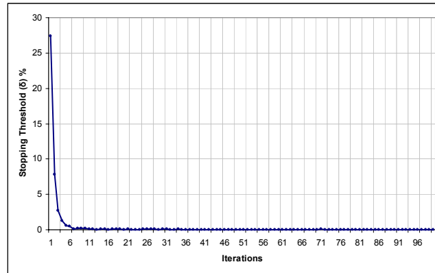
(e) Fig. 18 Time evolution of the Q (a), FOM (b), \gamma (c), \alpha_{ov} (d), and \delta (e) of the nonlinear diffusion for 100 iterations
