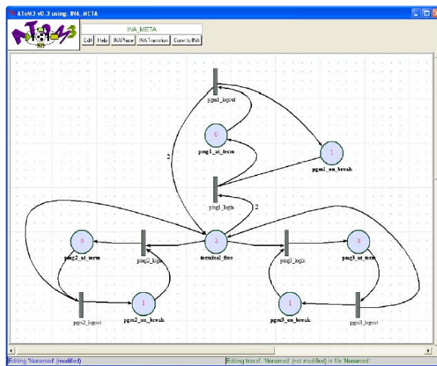
Fig. 6 3_prog_2_term problem created in our tool
