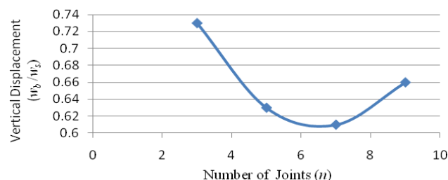
Fig. 5 The dependence of the number of bottom chord joints on displacements. w_b – vertical displacements of cable truss, w_s – vertical displacements of single cable, f_t – top chord camber, l – span
