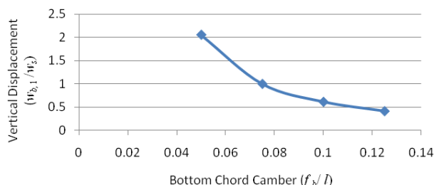
Fig. 4 The dependence of bottom chord camber on displacements. w_b – vertical displacements of cable truss, w_s – vertical displacements of single cable, f_t – top chord camber, l – span
