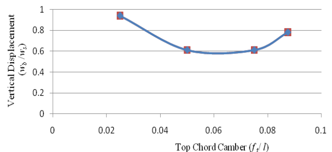
Fig.3 The dependence of top chord camber on displacements. w_b – vertical displacements of cable truss, w_s – vertical displacements of single cable, f_t – top chord camber, l – span
