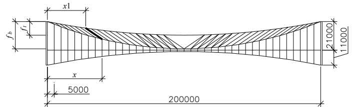
Fig.10 Parameters of cable truss
