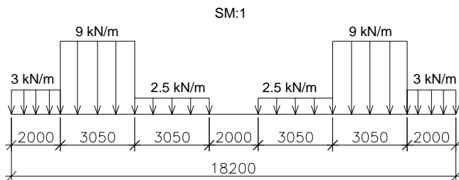
Fig. 9. Applied load to the bridge.
