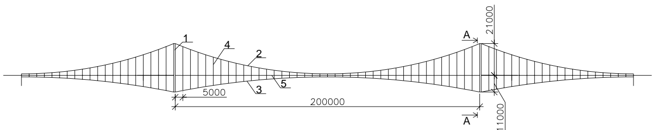
Fig.7 The bridge longitudinal view. 1 – Pylon of the bridge, 2 – Main load carrying cable, 3 – Stabilization cable, 4 – Suspensions, 5 – Deck
