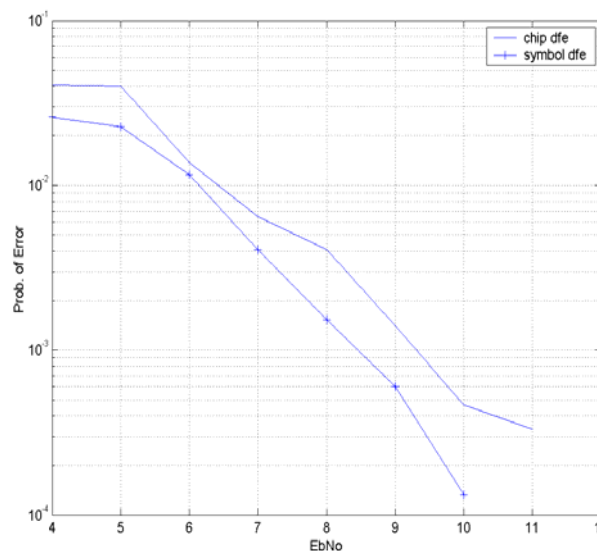
Fig. 5 Ninetieth-percentile probability of error for BCH (15,5)
