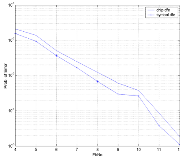
Fig. 4 Probability of error for BCH (15,5)
