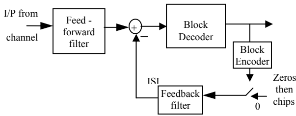
Fig. 2 Symbol DFE Block Diagram
