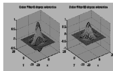
Fig. 5 Gabor filter
