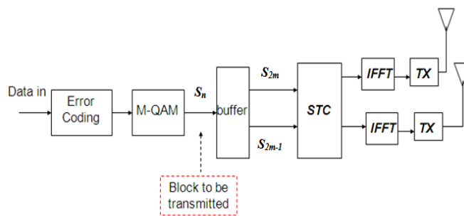
Fig. 3 Down Link: Transmit Diversity use Alamouti Space Time Coding
