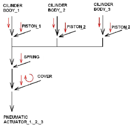
Fig. 8 Step diagram for assembly of pneumatic actuator
