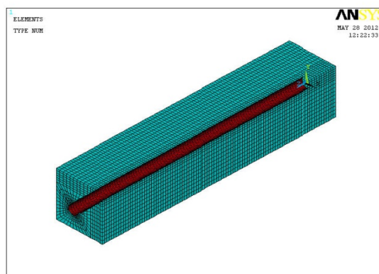
Fig. 7 Quarter model of RVE of CNT reinforced cement with 4 CNTs
