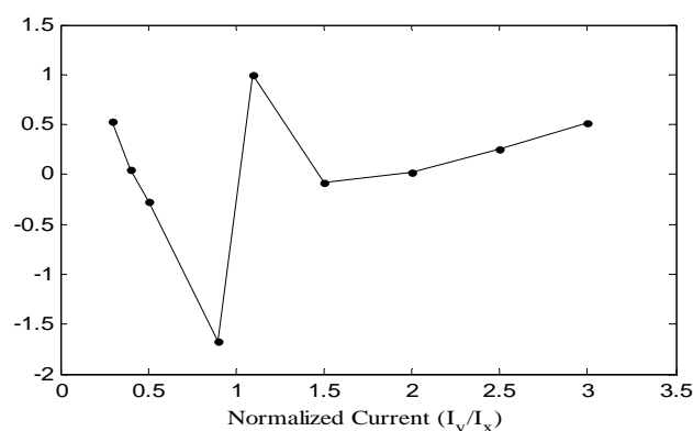
Fig. 4 Errors between the simulated and the theoretical results (@ I_{in} = 100 \text{ nA} )
