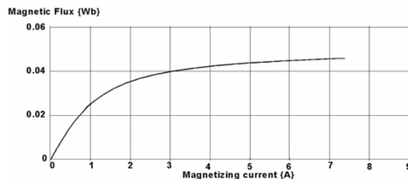
Fig. 8. Saturation curve of equation (42).
