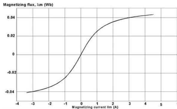
Fig. 9. Nonlinear performance of the transformer of Fig. 6.
