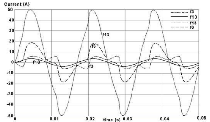
Fig. 16. Transformer response with three windings.
