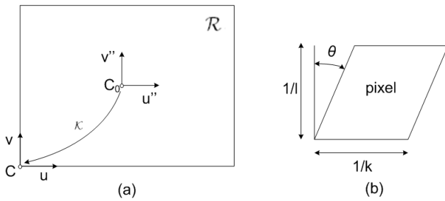
Fig. 1. Ascendence of intrinsic parameters during image transformation from normalized image plane into projective plane (a) and pixel form after rotation of coordinate systems of normalized image plane and projective plane (b).
