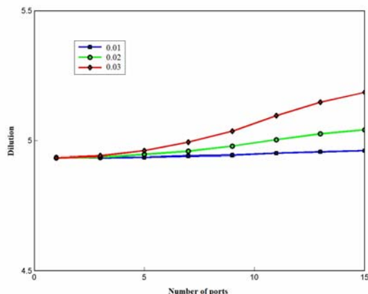
Fig. 6 Dilution for a parallel line diffuser discharge
