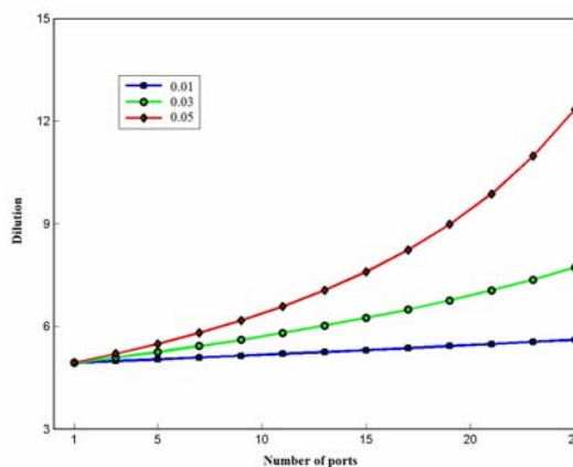
Fig. 5 Dilution for a perpendicular line diffuser discharge
