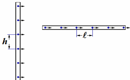
Fig. 4 Multiport line diffuser designs: Perpendicular (left) and parallel (right) to the direction of current
