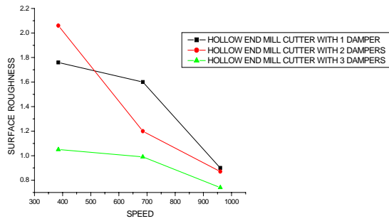
Fig. 4 Variation of Surface roughness with speed
