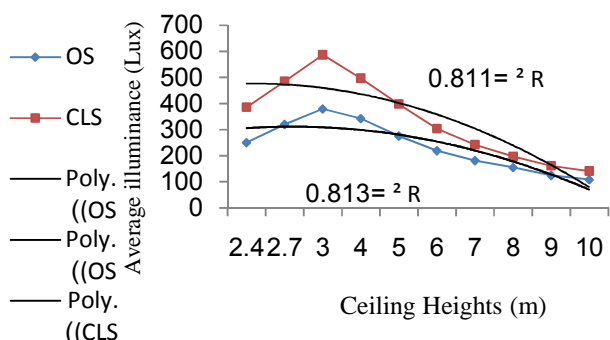
Fig. 6 Average illuminance ratio versus multiple ceiling and higher window heights under an overcast and cloudy sky
