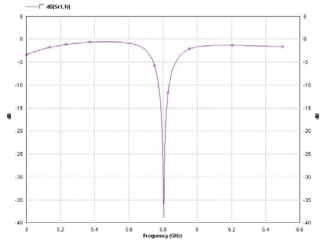
Fig. 5. Return loss for geometry 1
