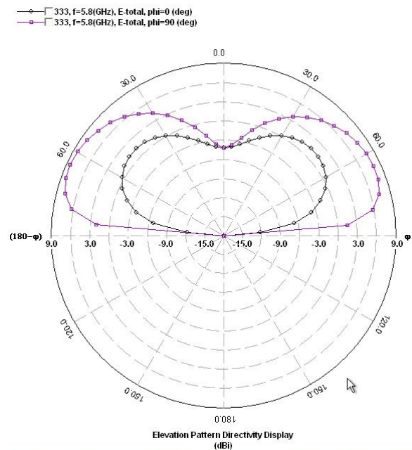
Fig. 7. Radiation pattern for geometry 1
