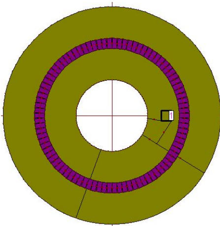
Fig. 3. Geometry of Antenna design 2
