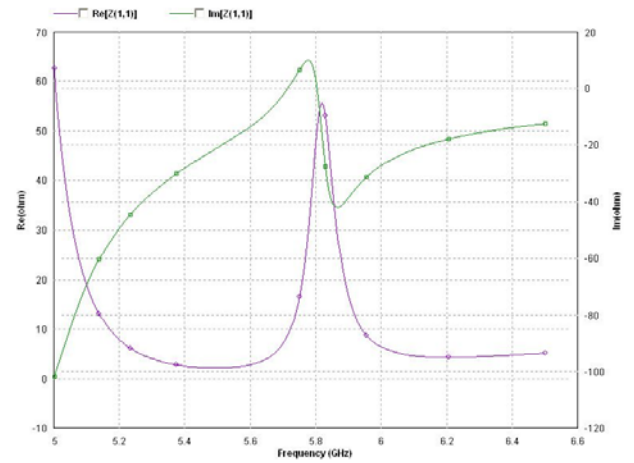
Fig. 6. Zin for geometry 1
