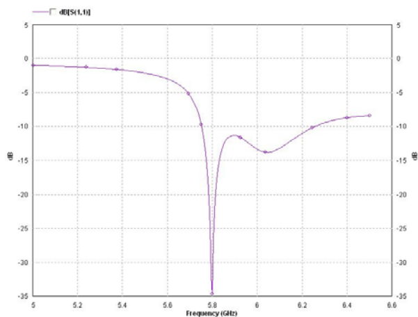
Fig. 8. Return loss for geometry 2
