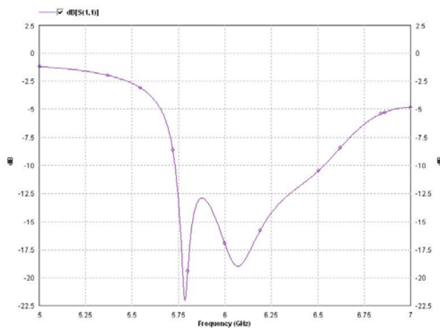
Fig. 11. Return loss for geometry 3
