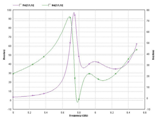
Fig. 9. Zin for geometry 2
