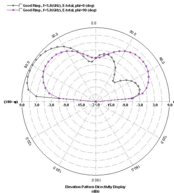
Fig. 10. Radiation pattern for geometry 2
