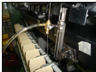
Fig. 3 Transferring the compressed air into the nozzle
