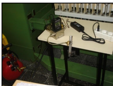
Fig. 5 Measurements by electronic mass flow meter
