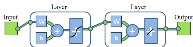
Fig. 2 Neural Network Model Structure of Grass Carp Hemorrhage Predication
