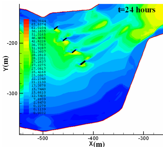
Fig. 8 Shear stress field around the bridge piers for Q=914.63 m 3 /s.
