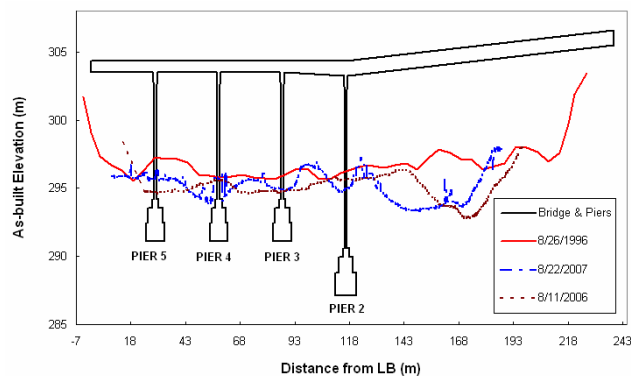
Fig. 2 Surveyed upstream cross section and pier soundings at bridge 524, Tanana River at Big Delta, Alaska.
