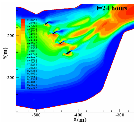
Fig. 7 Flow velocity field around the bridge piers for Q=914.63 m 3 /s.
