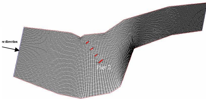
Fig. 4 Calculation grid used for the 3D hydrodynamic modeling by SSIIM program.
