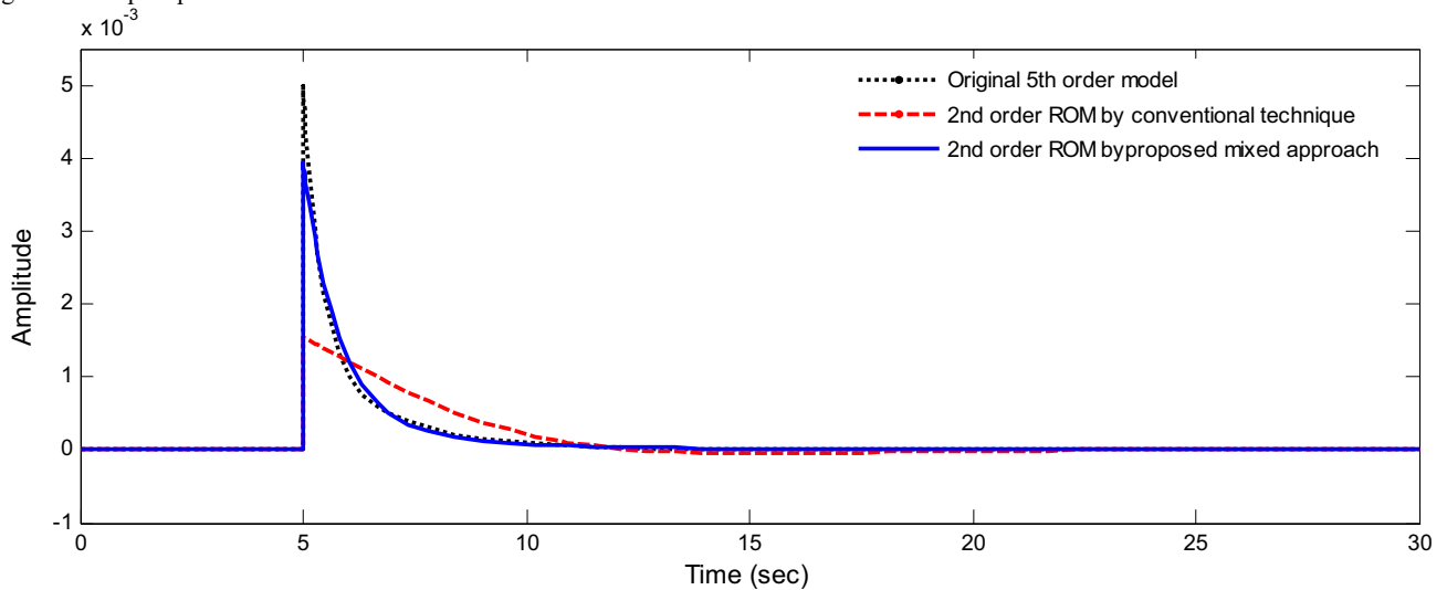
Fig. 5. Unit impulse response
