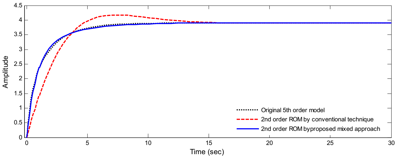
Fig. 4 Unit step response
