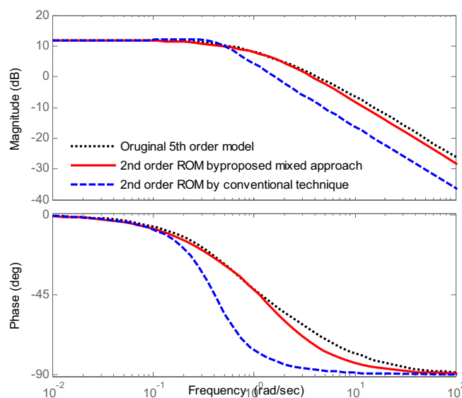
Fig. 6. Frequency response
