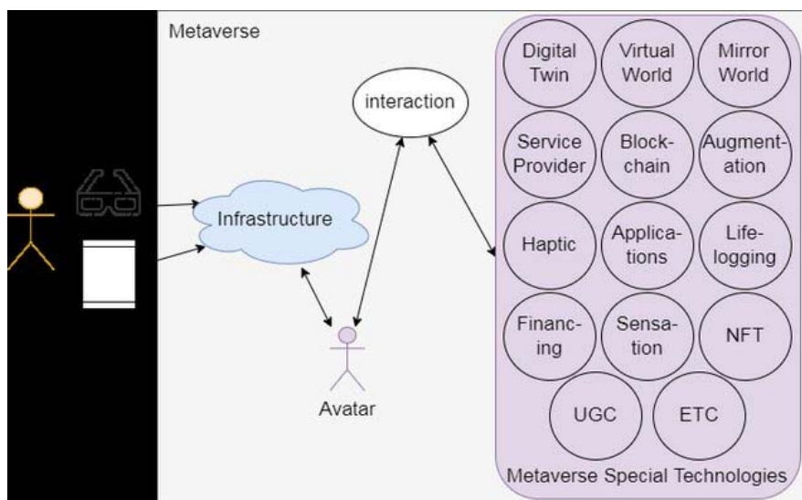
Fig. 1 Metaverse framework [2]
