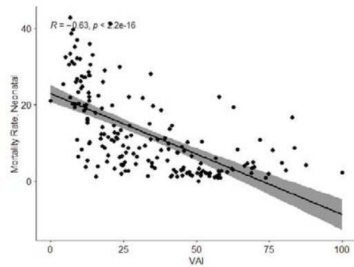
Fig. 13 Scatterplot of VAI and the neonatal mortality rate, with all countries
