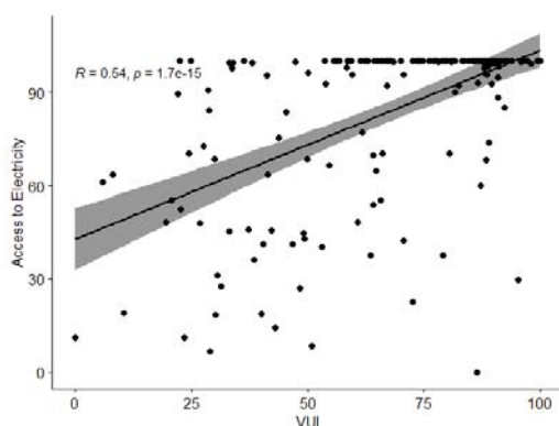
Fig. 9 Scatterplot of VUI and access to electricity, with all countries
