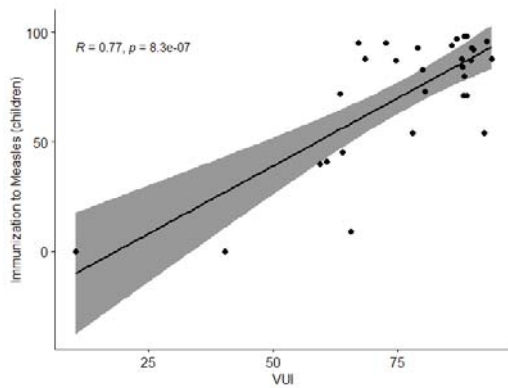
Fig. 11 Scatterplot of VUI and immunization to measles in children, with the top 30 populated countries
